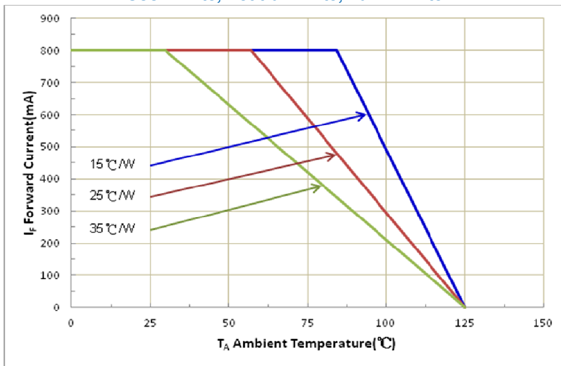
Current Derating Curve for 800mA Drive Current Cool-White, Neutral-White, Warm-White
