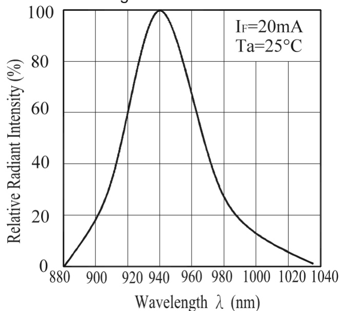
Fig.2 Relative Radiant Intensity vs. Wavelength
