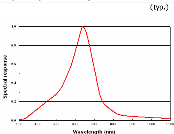
Fig.3 Spectral Response
