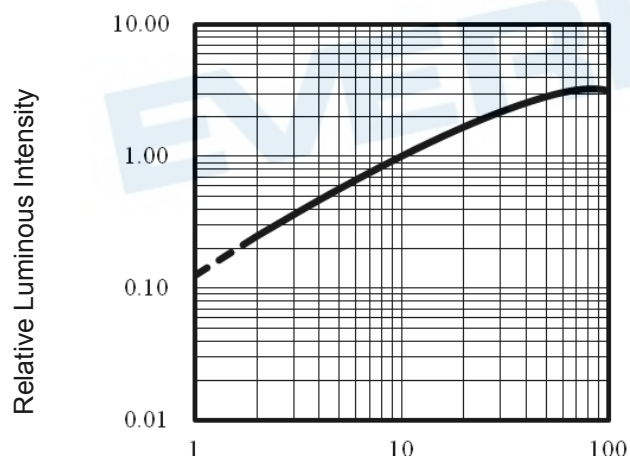
Relative Luminous Intensity vs. Forward Current (Ta=25°C)
