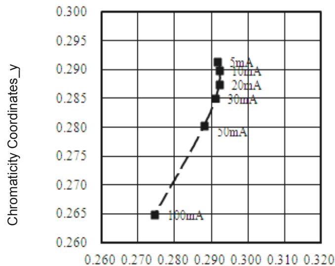
Chromaticity Coordinates vs. Forward Current (Ta=25°C)
